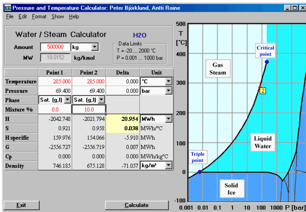
Figure 3: Evaporation process.
