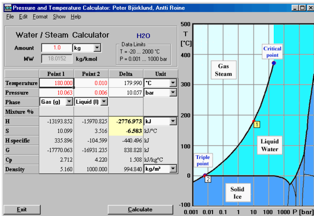
Figure 1: Pressure-Temperature calculator for water.
