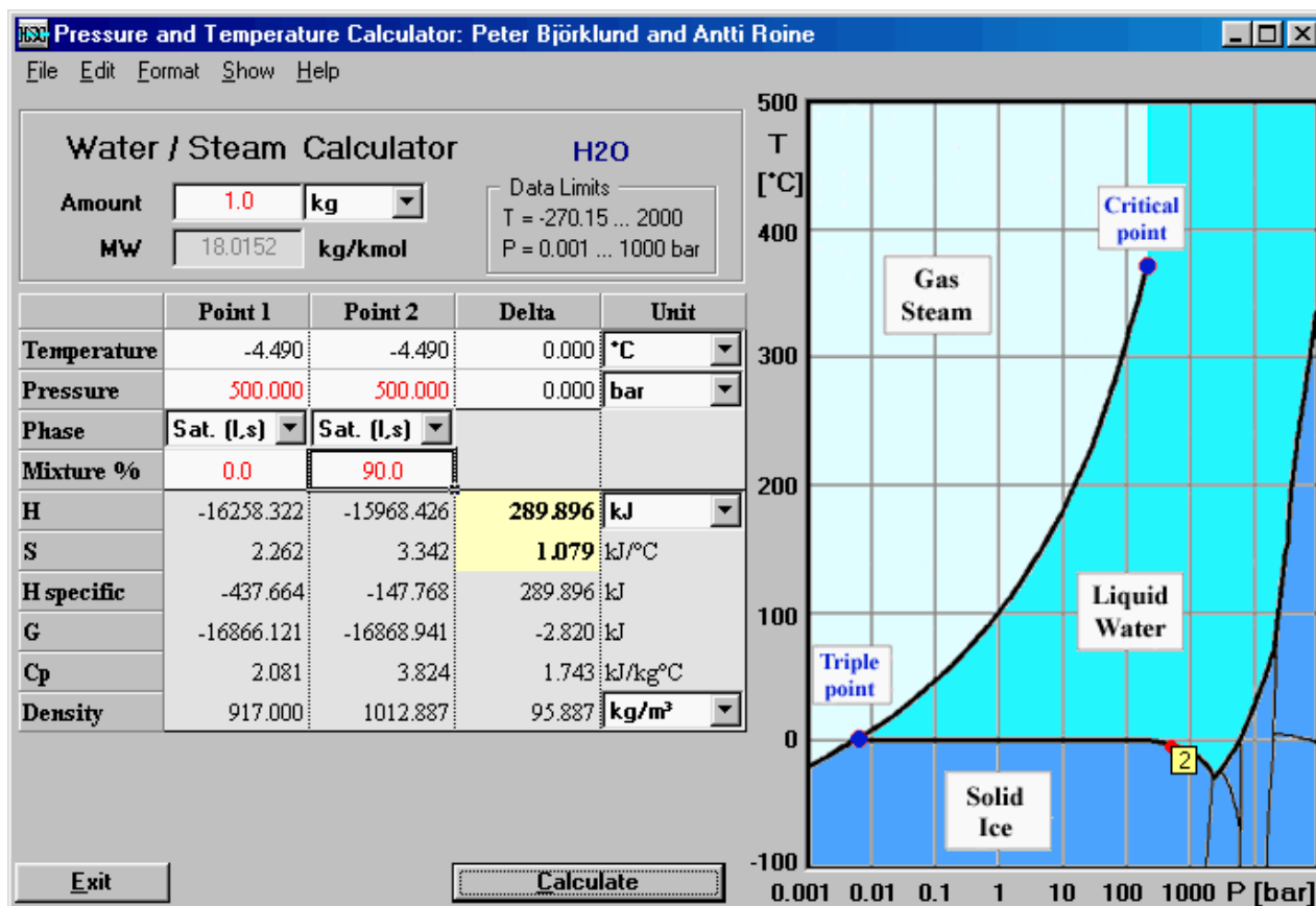
Figure 2: Melting of ice at a pressure of 500 bar.
