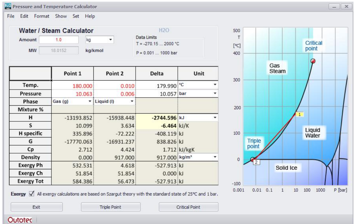
Fig. 1. Pressure-Temperature calculator for water.
